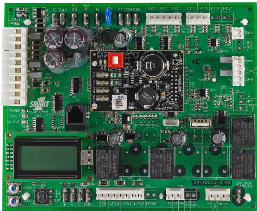
Single Stage with Optional Communication Board
